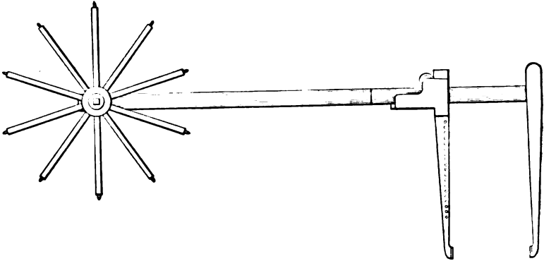
FIG. 2.—Wheel for Measuring Lengths of Logs.
