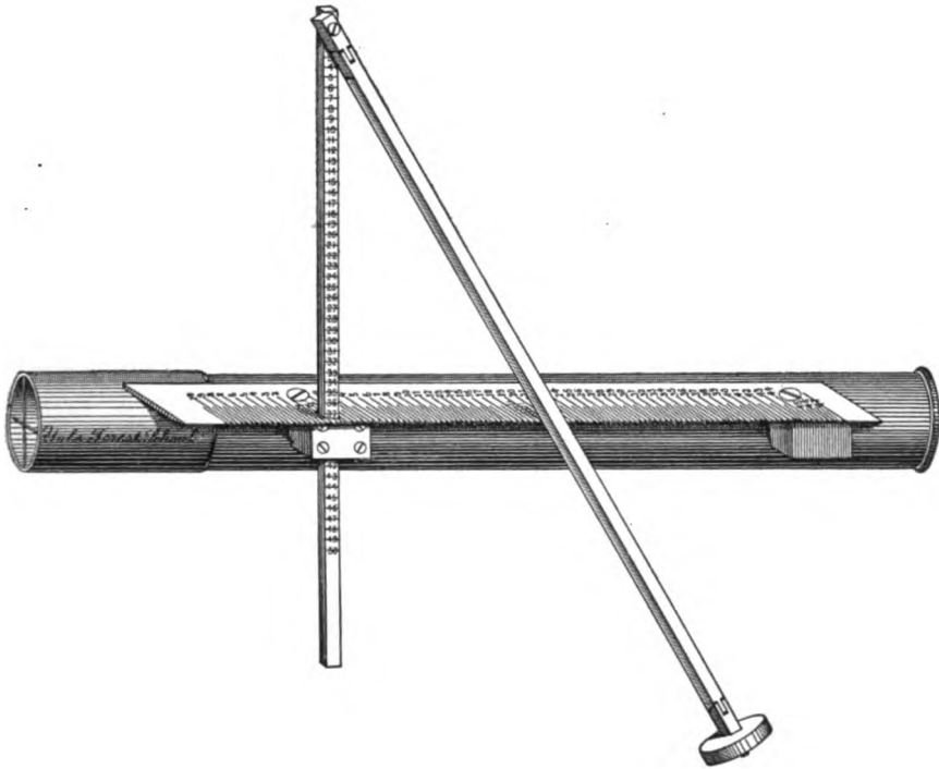
FIG. 21.—The Weise Height Measure.
