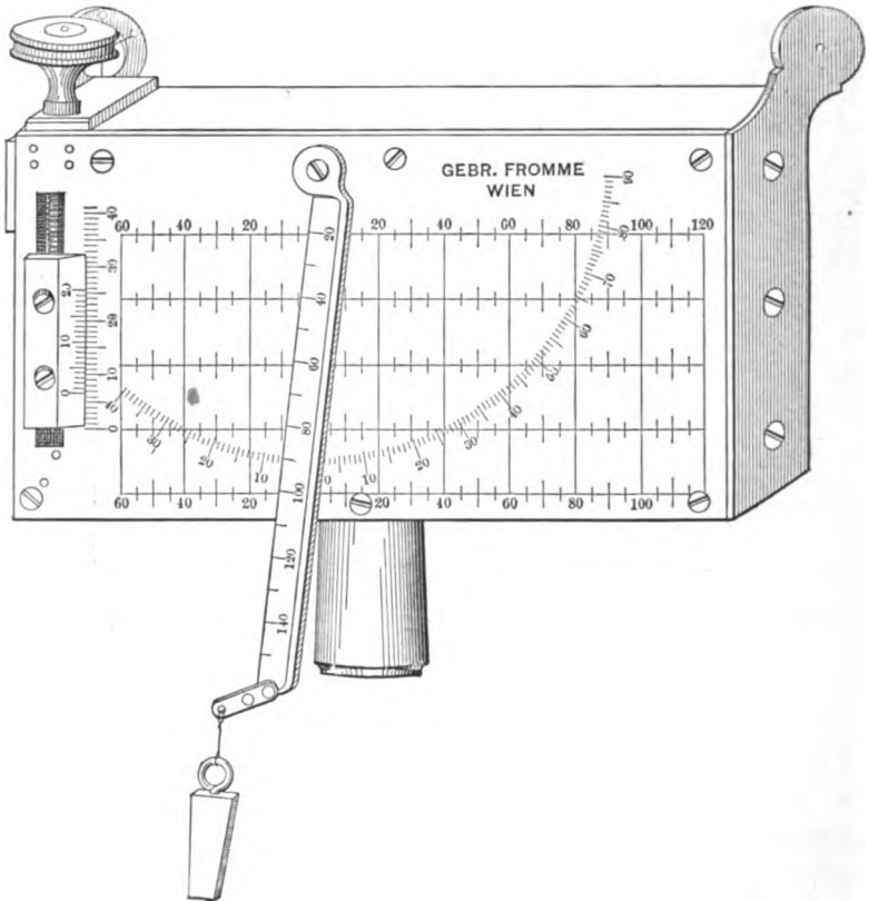
FIG. 26.—The Winkler Height Measure.
