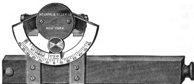
FIG. 32.—The Abney Hand Level and Clinometer.
