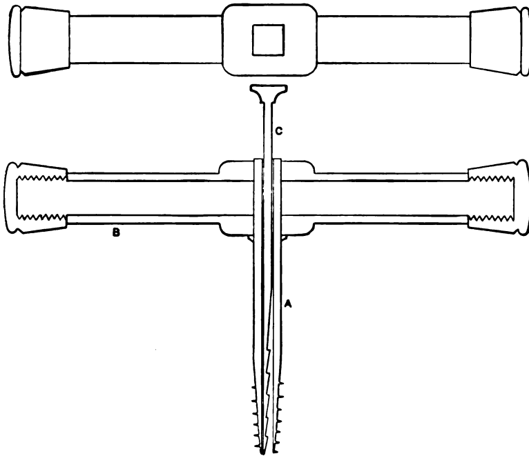
FIG.45.—Pressler's Increment Borer.
