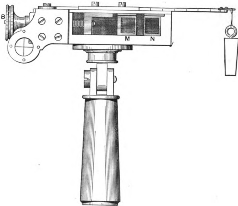
FIG. 27.—The Winkler Instrument used as a Dendrometer.
