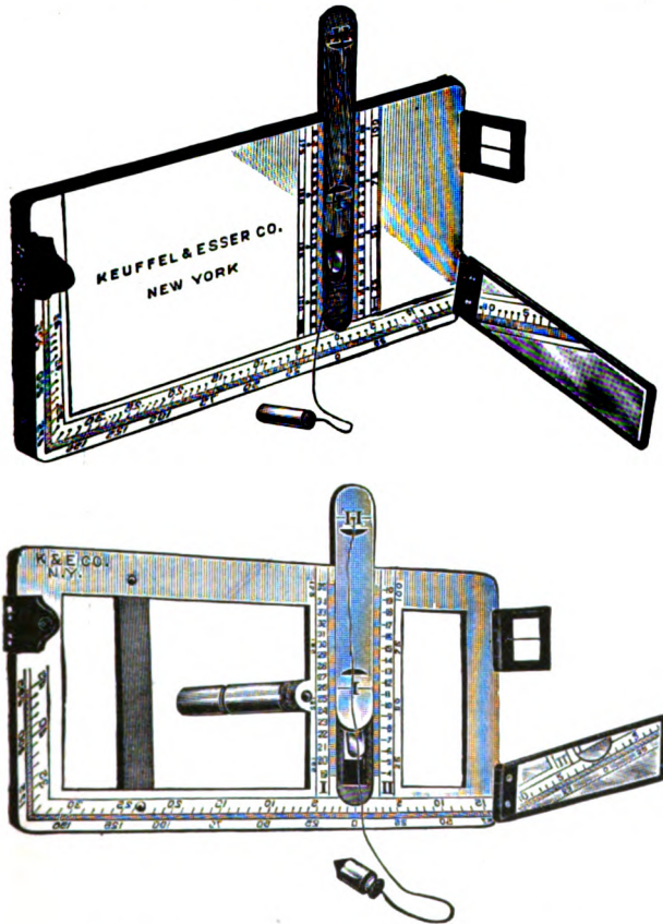
FIG. 15.—The Faustmann Height Measure.
